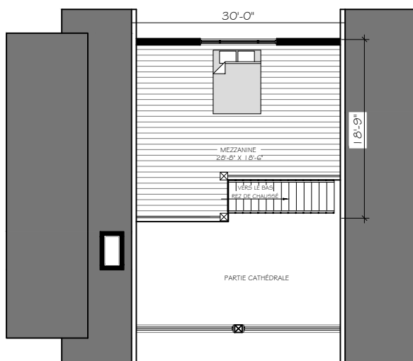
MEZZANINE
